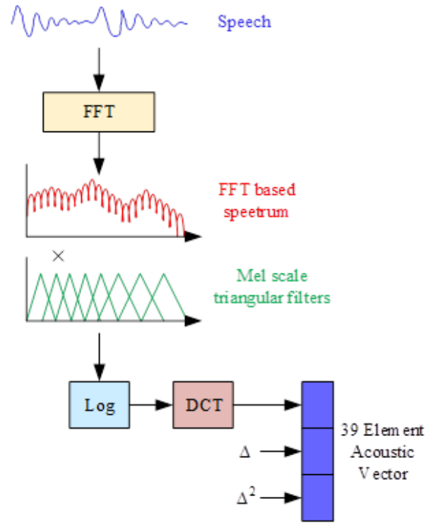
Figure 1: Based on MFCC front-end processing
