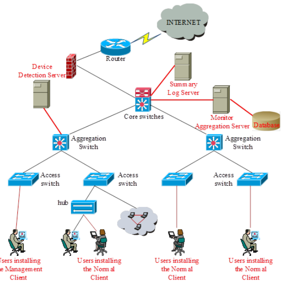
Figure 5: Network department
