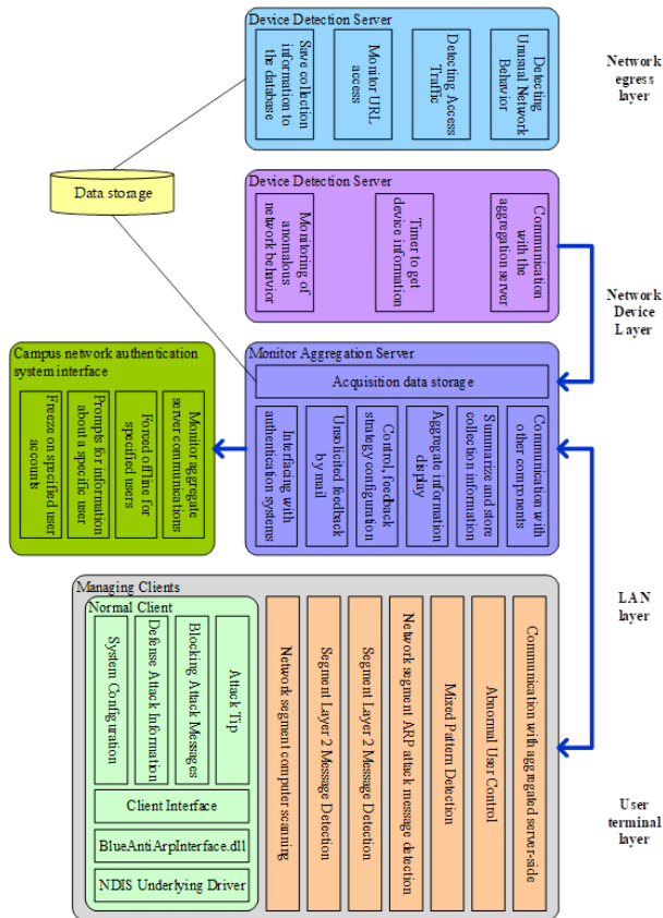
Figure 4: System framework
