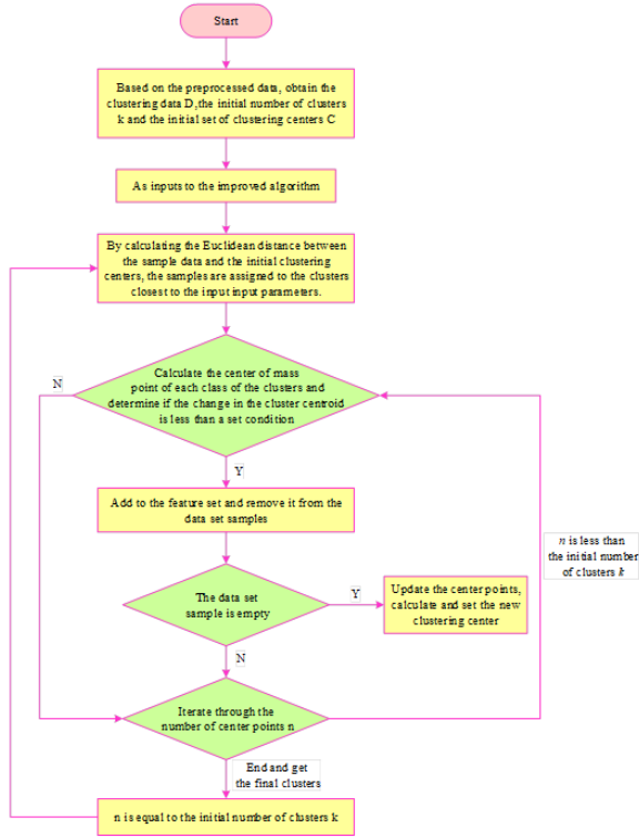
Figure 2: The computing framework of the integrated algorithm
