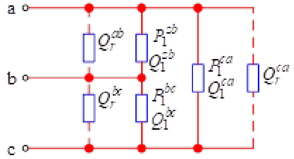
Figure 6: Reactive compensation for three-phase load power supply
