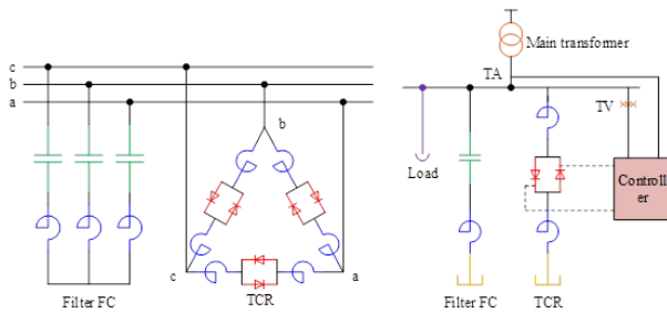
Figure 3: 3 TCR+ fc type SVC typical wiring diagram
