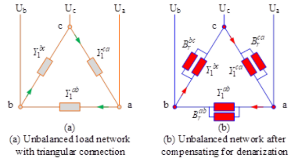
Figure 4: Compensation for the three-phase uneven load
