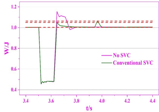
(a) Target 230kv bus power
