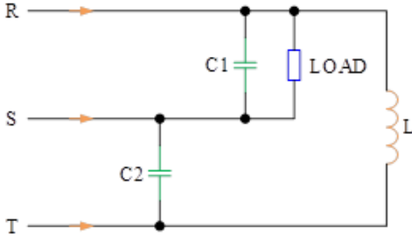
Figure 5: Reactive compensation for single-phase load power supply
