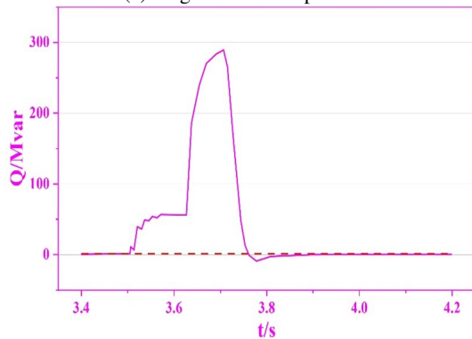
(b) SVC has no power output
