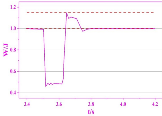
(a) Target 230kv bus power
