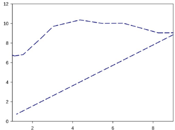
Figure 7: Reported impulse-response analysis for the estimated VAR model.
