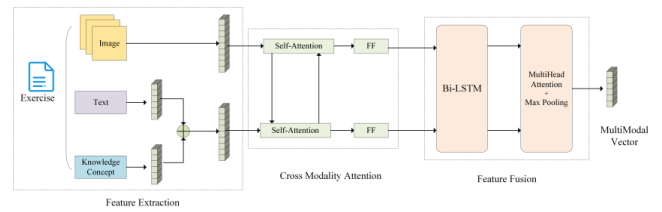
Figure 4: Multimodal fusion model
