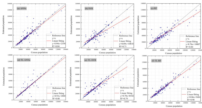
Figure 6: Performance Comparison of Six Machine-Learning Models for Estimating Urban Population Based on Economic and Industrial Features. Top Row: Baseline Models—ANN (a), SVR (b), and RF (c); Bottom Row: Transfer-Learning-Enhanced Models—TL-ANN (d), TL-SVR (e), and TL-RF (f). The Dashed Line Represents the Ideal Fit ( y = x ), While the Red Line Represents the Linear Regression Fit and Indicates Goodness of Fit
